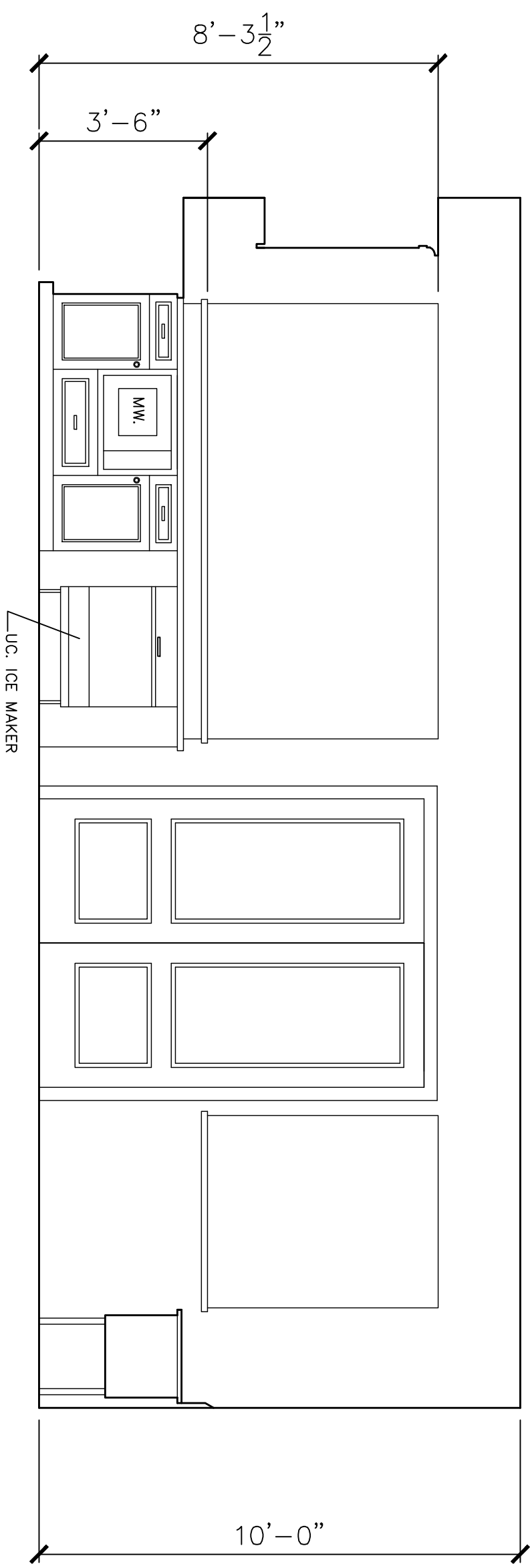
4 KITCHEN 3/8"=1'-0"
