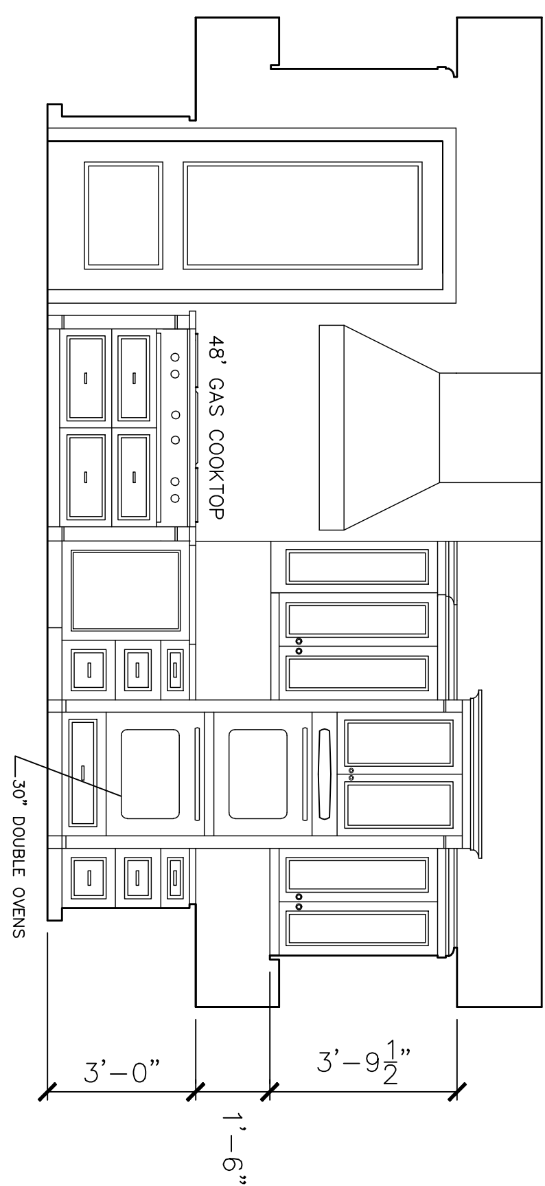
2 KITCHEN 3/8"=1'-0"
